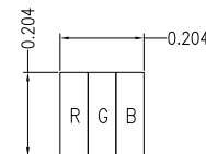
PIXEL DETAIL (SCALE 100:1)
